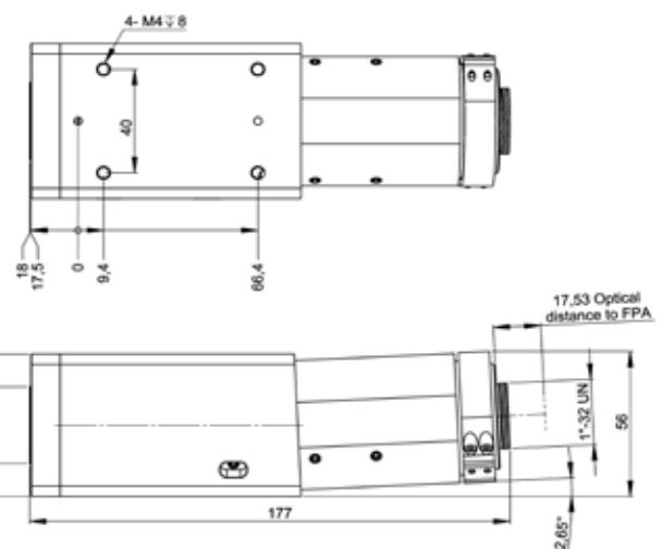
ImSpector V8E/V10E mechanical dimensions
