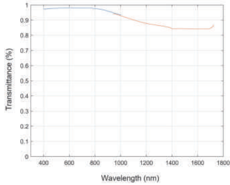
Acrylic Window - double sided anti-reflexion coating
