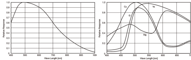
Sensor specifications b/w; color (extracted from the data sheet of the sensor - excluding lens and filter)
