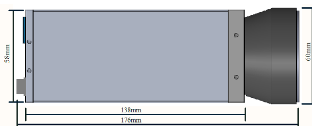
Top View Dimensions
