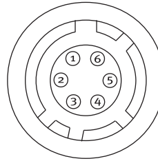
HIROSE HR10A-7R-6P
